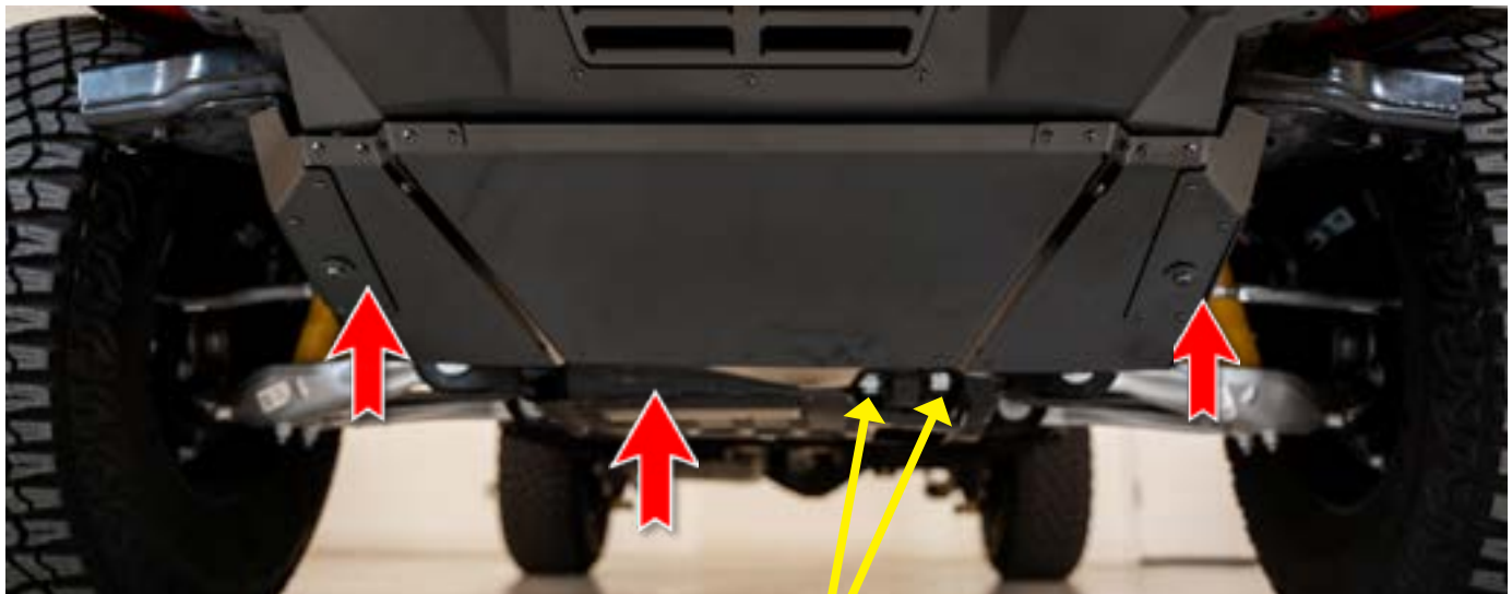
18mm bolts
