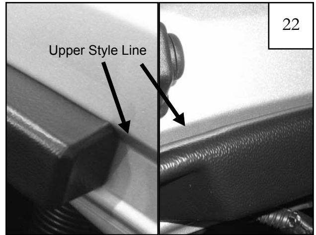
Picture on left: Top edge of inner piece along upper style line Picture on right: Top edge of inner piece tucked below upper style line; this forcibly angles and deforms inner pieces and flare is difficult or impossible to install
