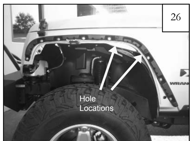
Secure inner pieces D7 (and P7 for passenger side installation) to the sheet metal using the following 2 Steps: Step 1 Position inner piece on fender, aligning with existing holes in first two inner pieces.
