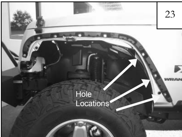
Secure inner pieces D2 (and P2 for passenger side installation) to the sheet metal using the following 3 Steps: Step 1 Position inner piece on fender, aligning with existing factory holes in sheet metal.
