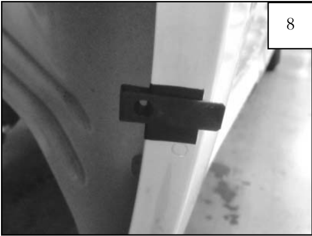
Install a Clip (CL1-0009) over each of the four Tabs (MT1-0034) placed over the upper 4 marks made in Step 16.
