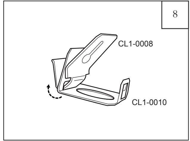
8 Assemble Clip CL1-008 with CL1-0010 as indicated in the above diagram. Insert tab of CL1-0008 through slot in CL1-0010.
