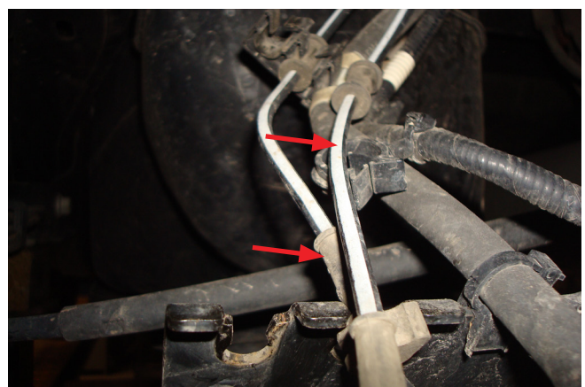
Pull the ABS lines out and away from the left side of the bracket bolted to the axle. Fig. 13
