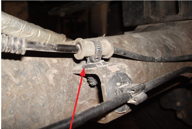
Pull the tree mount holding the ABS line, out of the top mounting of the bracket. Fig. 10
